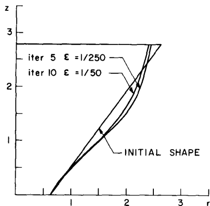
Fig. 12. Optimal diffusers for L = 2.775 .
