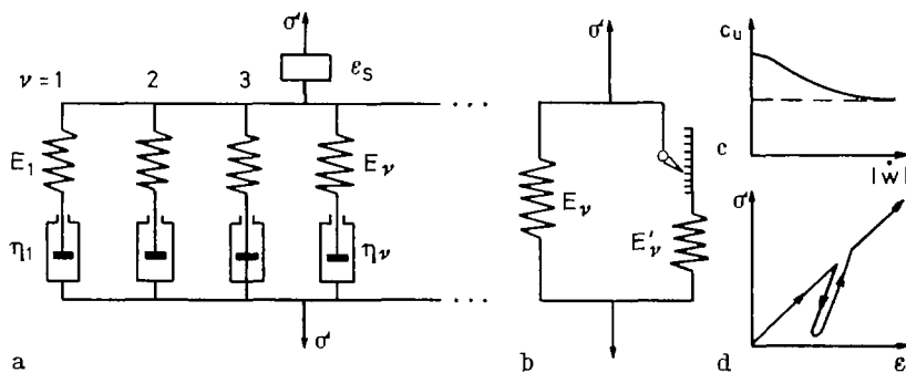
Fig. 3. a Maxwell chain model with shrinkage strain; b Ratchet model (b-d)
