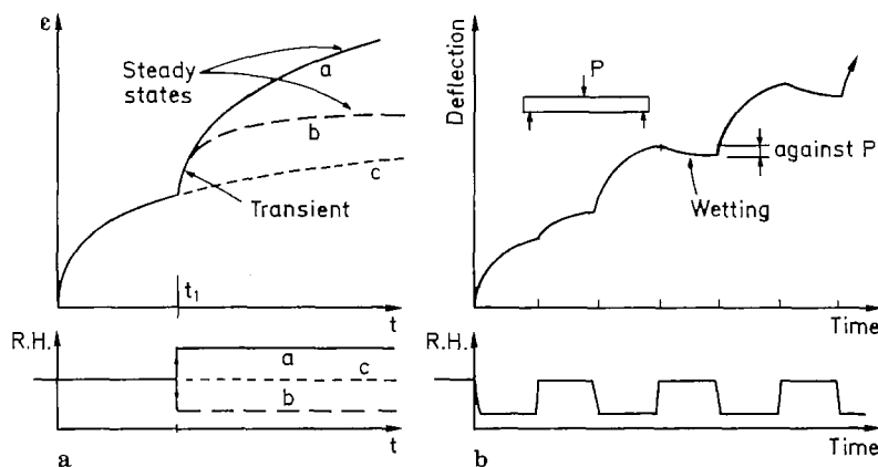
Fig. 4. a Creep after a decrease or increase of relative humidity; b typical deformations at humidity changes
