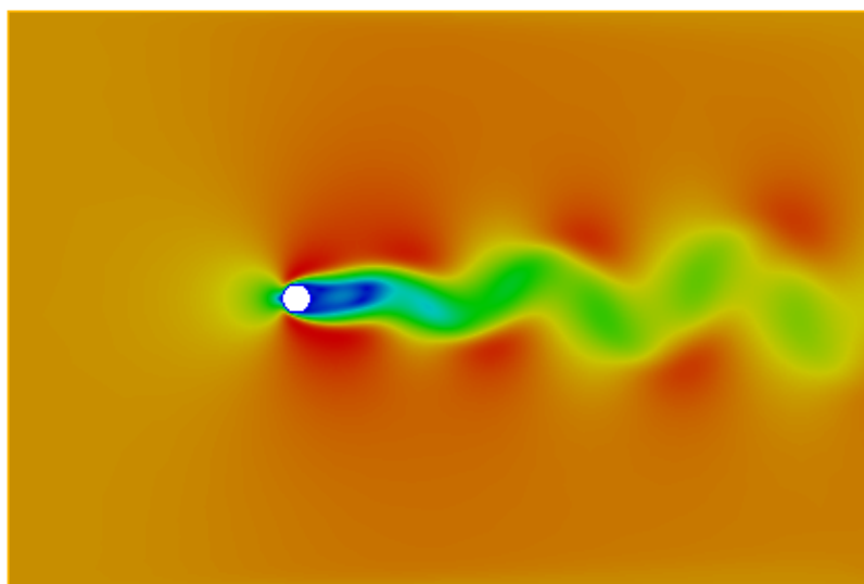
Figure 7. The discrete velocity \mathbf{u}_h .
